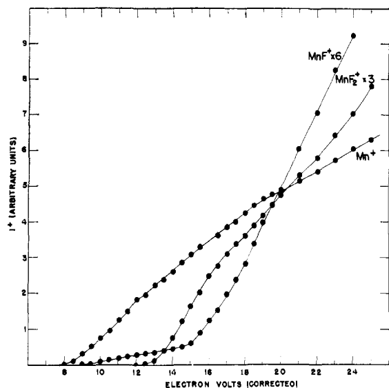
Fig. 3.—Ionization efficiency curves for species observed over \text{MnF}_2\text{-Mn} .
