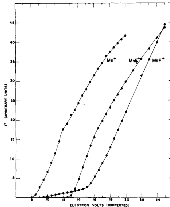
Fig. 2.—Ionization efficiency curves for species observed over \text{MnF}_2 .
