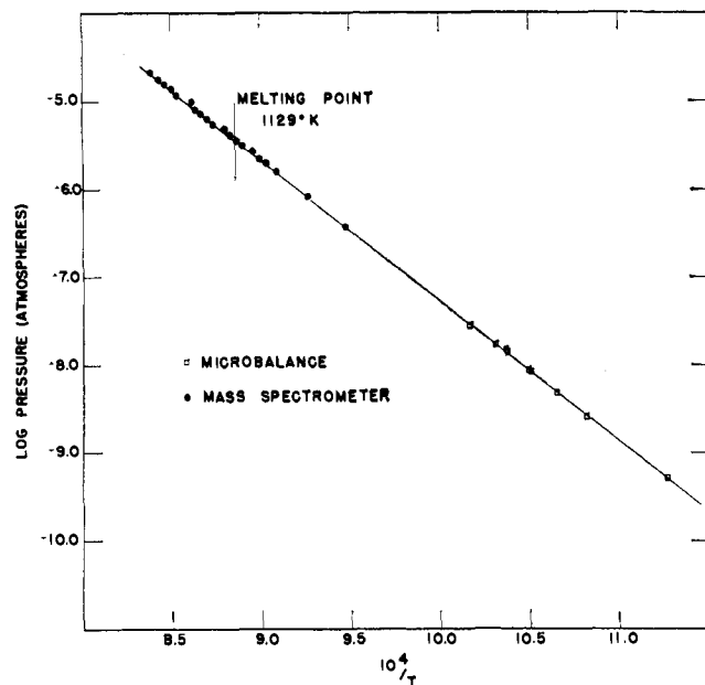
Fig. 1.—Vapor pressure data for \text{MnF}_2 .
